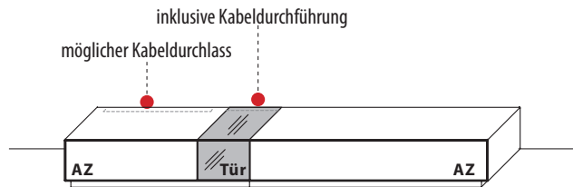
B 257,5 cm x H 29,0 cm x T 55,0 cm (2 Elemente)
