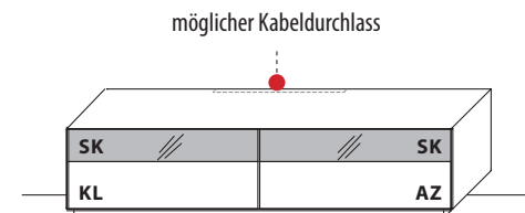
B 193,5 cm x H 45,0cm x T 55,0 cm
